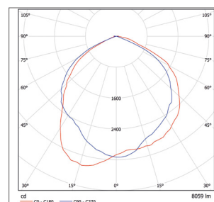
COBRA LED-L-97K60-MV
